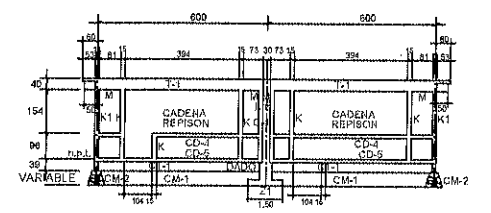
FACHADA ESTRUCTURAL PRINCIPAL
