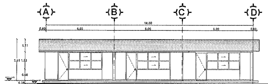
ALZADO PRINCIPAL
