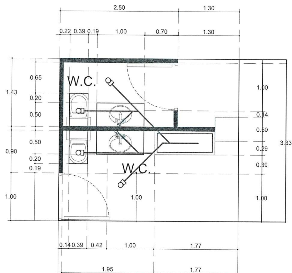
IS PLANTA SANITARIA BAÑOS 1/100
