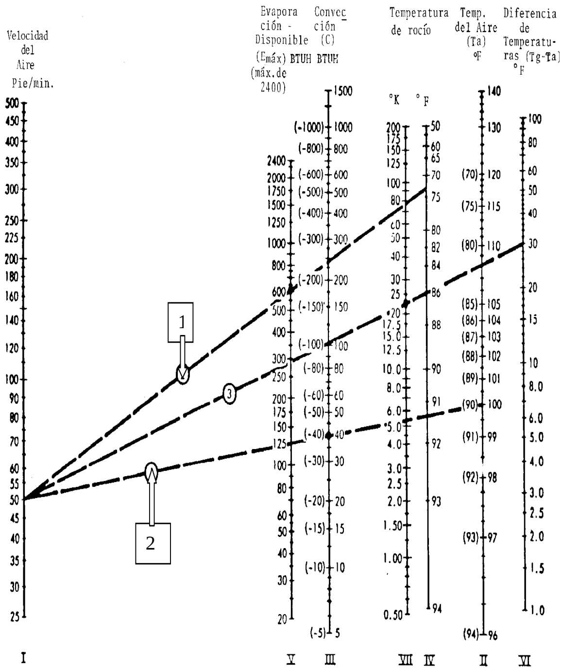
NOMOGRAMA No.1
